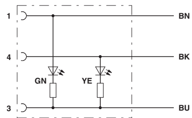
Contact assignment of M8 socket with 2 LEDs
